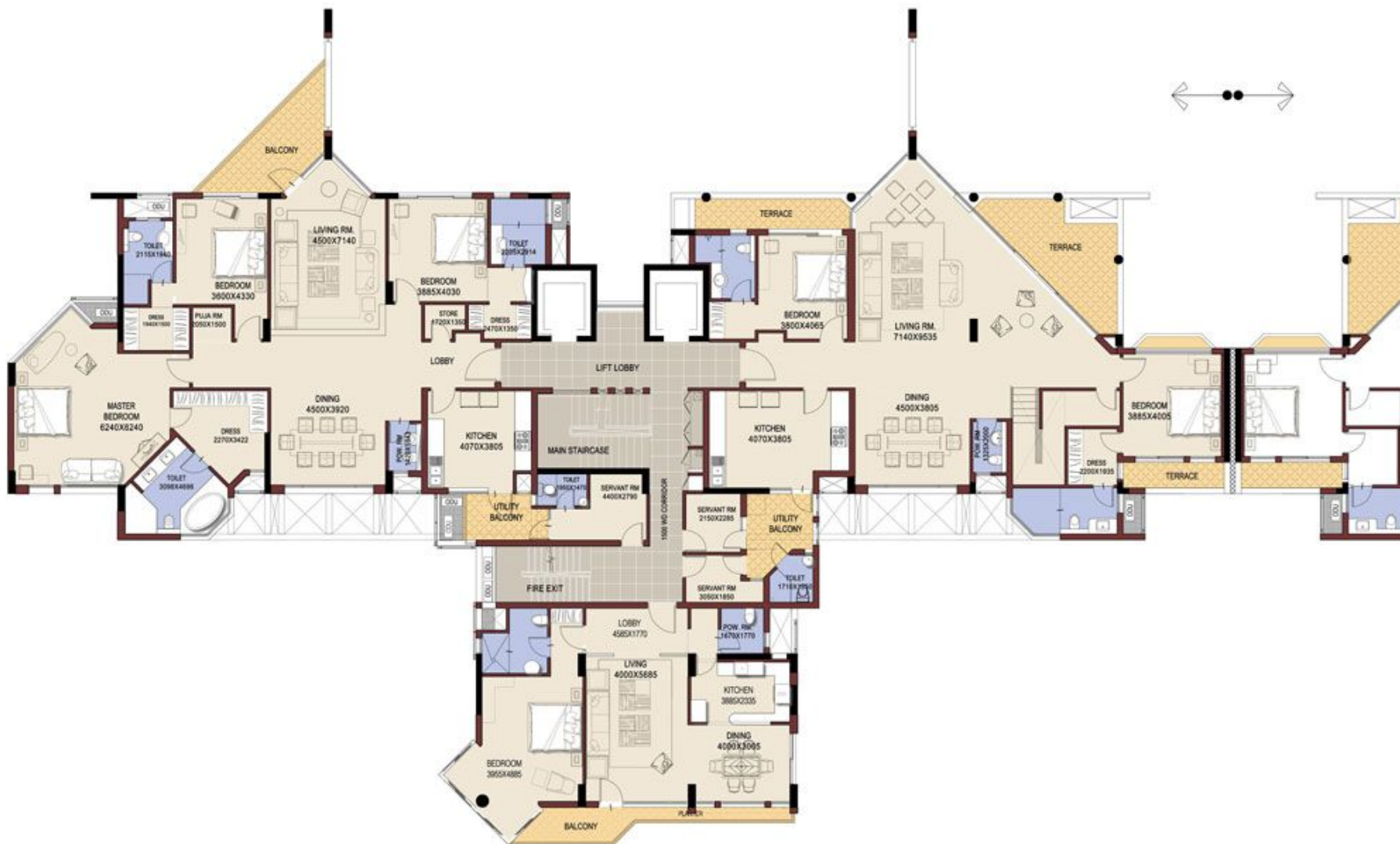
13TH FLOOR PLAN-TOWER 1 DUPLEX PENTHOUSE (LOWER LVL)
